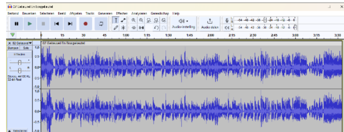
Audacity
